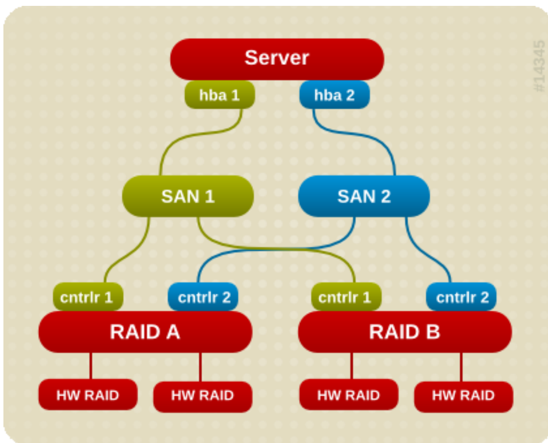
Figure 1.2. Active/Passive Multipath Configuration with Two RAID Devices
