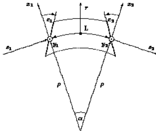
Figure 3: Reference System for Sector Bends; The signs of the pole-face rotations are positive as shown.
