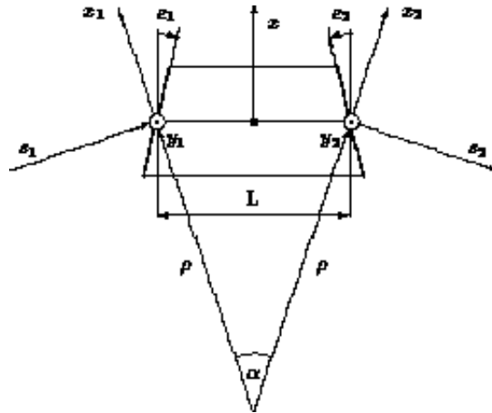
Figure 2: Reference System for Rectangular Bends; The signs of the pole-face rotations are positive as shown.
