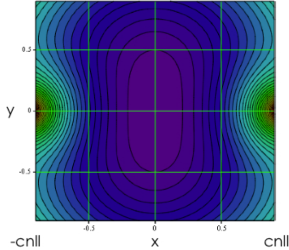
Figure 10.1: Contour plot of the scalar potential
