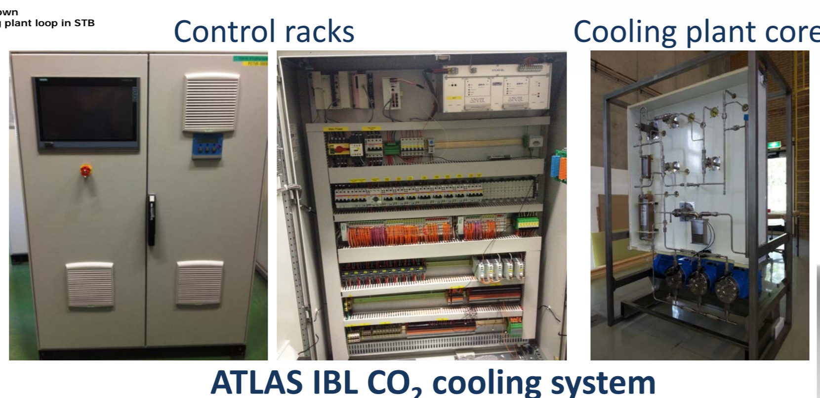
ATLAS IBL CO 2 cooling system
