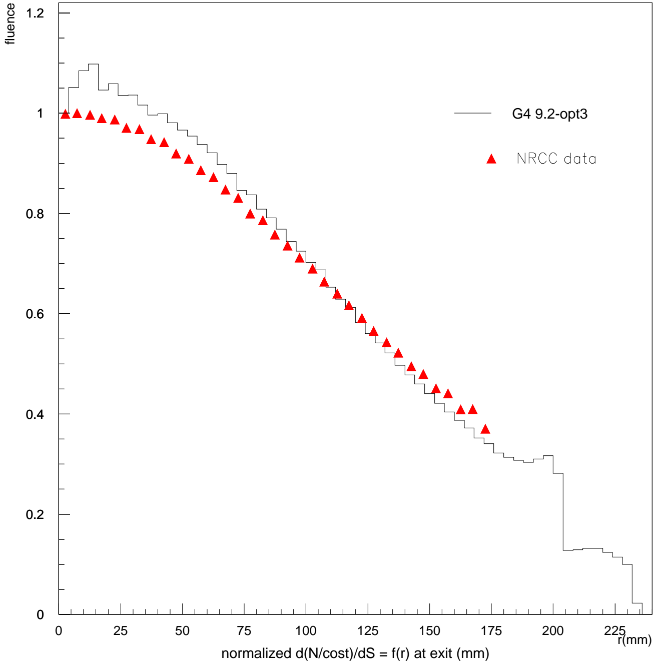
dFluence/ds distribution of 13 MeV e- in Au3
