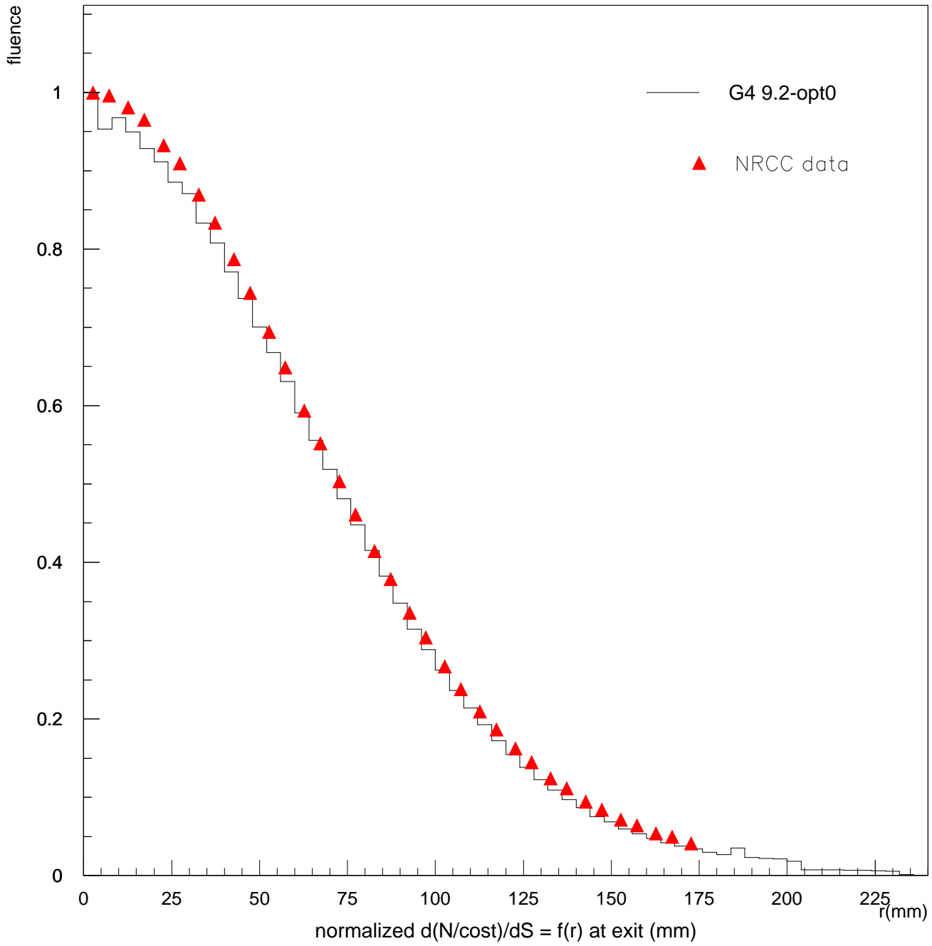
dFluence/ds distribution of 13 MeV e - in Ti4
