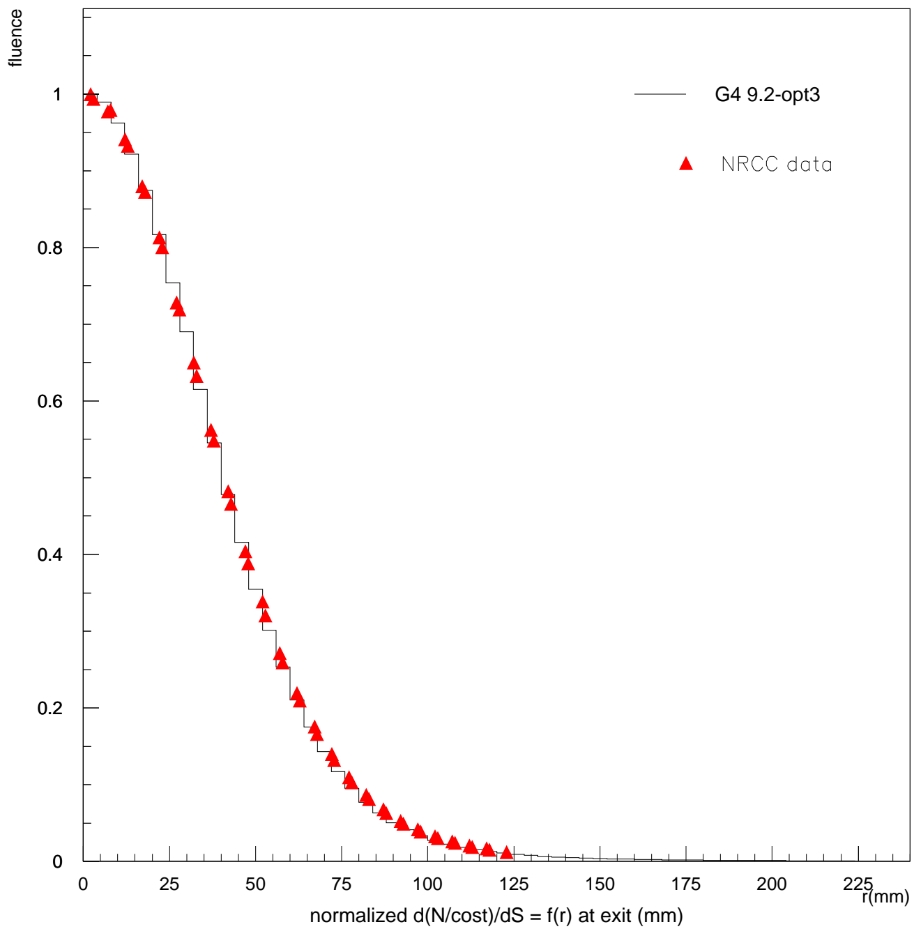
dFluence/ds distribution of 13 MeV e- in nofoil
