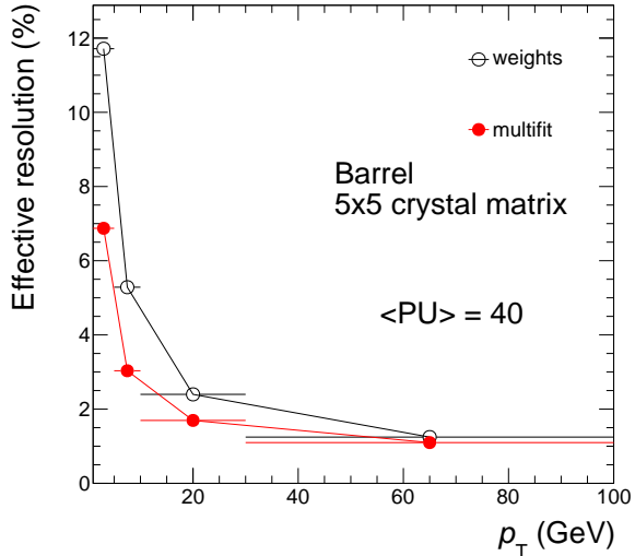
CMS Simulation (13 TeV)
