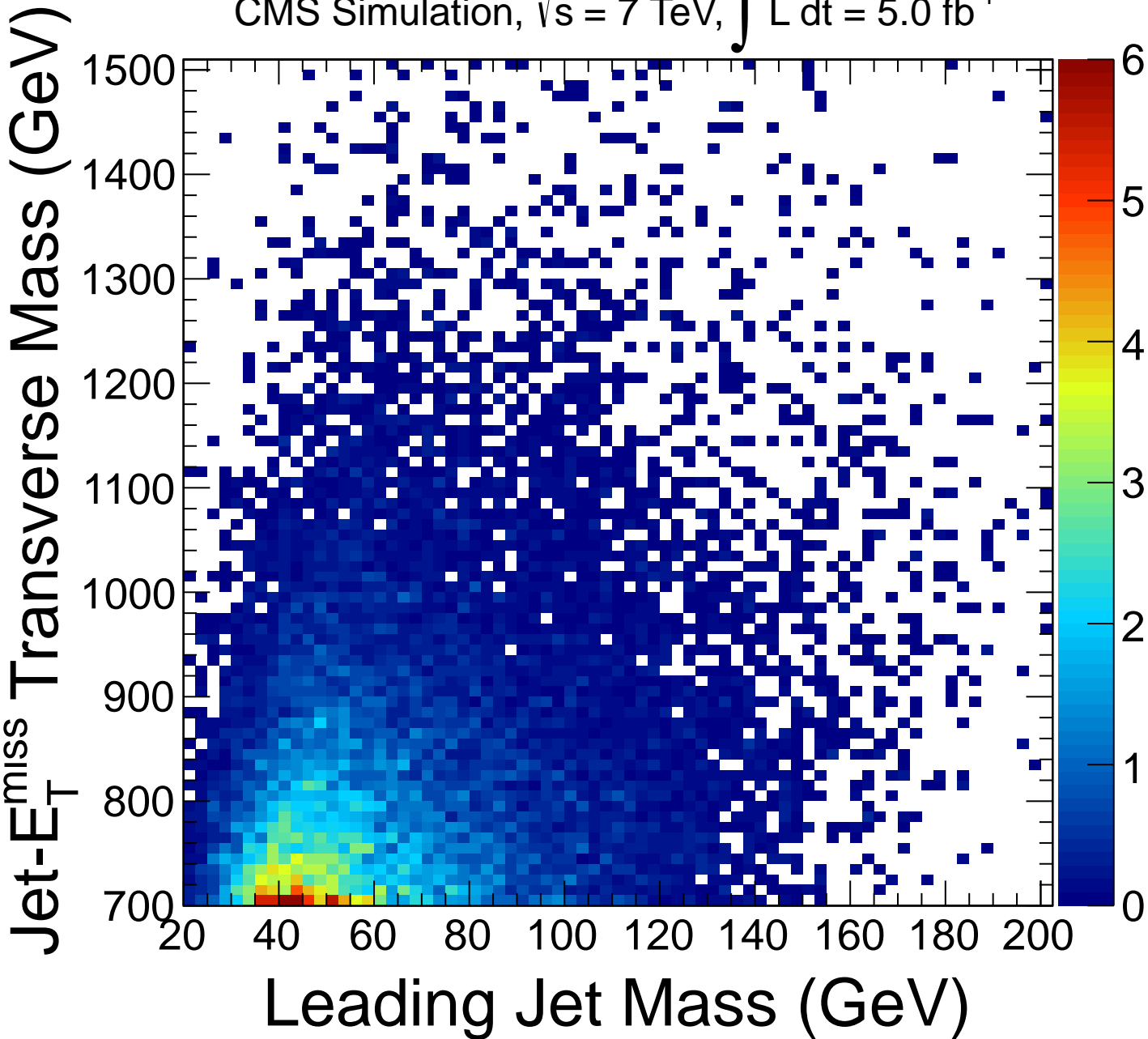
(a) Standard Model
