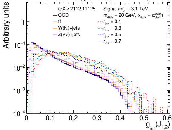
CMS Simulation Supplementary (13 TeV)
