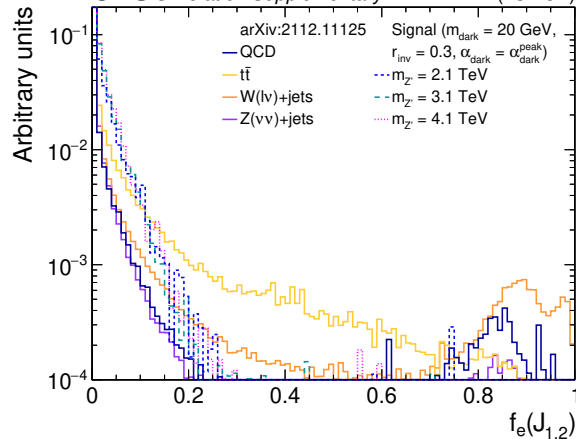
CMS Simulation Supplementary (13 TeV)
