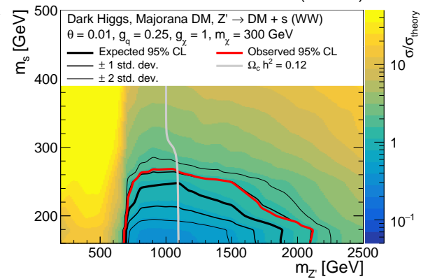
CMS 138 fb -1 (13 TeV)
