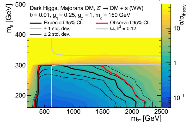
CMS 138 fb -1 (13 TeV)
