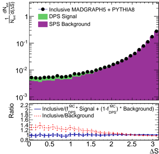
CMS Simulation, pp \rightarrow W + \text{jets} , \sqrt{s} = 7 \text{ TeV}
