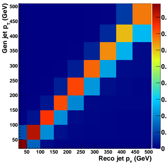
CMS Simulation pp \rightarrow 2b + 2j + X
