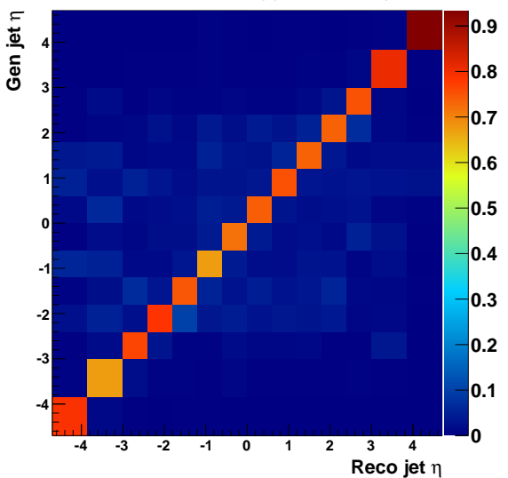
CMS Simulation pp \rightarrow 2b + 2j + X
