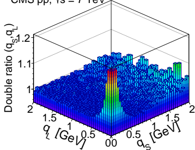
CMS pp, \sqrt{s} = 7 TeV
