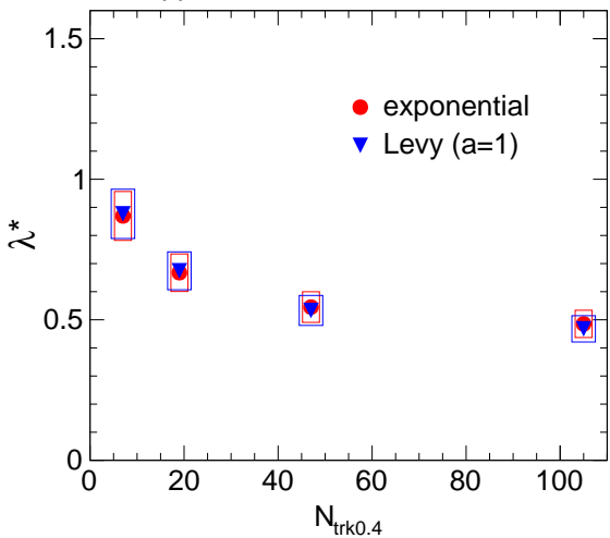
CMS pp, \sqrt{s} = 7 TeV
