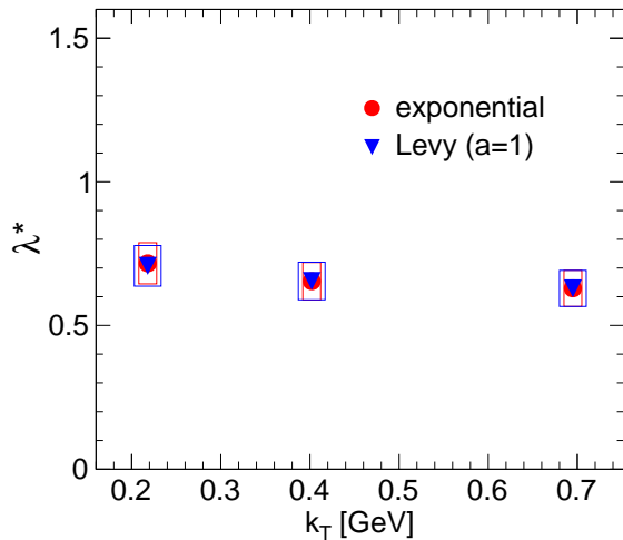
CMS pp, \sqrt{s} = 7 TeV
