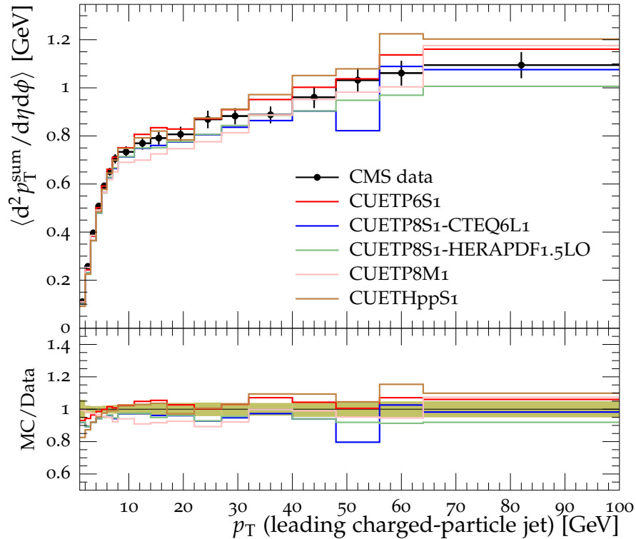
TransAVE p_T^{\text{sum}} density, \sqrt{s} = 2.76 TeV
