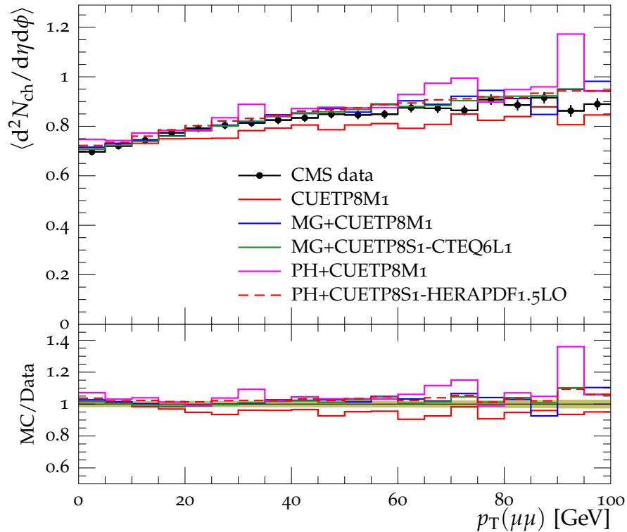
Toward N_{\text{ch}} density vs p_{\text{T}}(\mu\mu)
