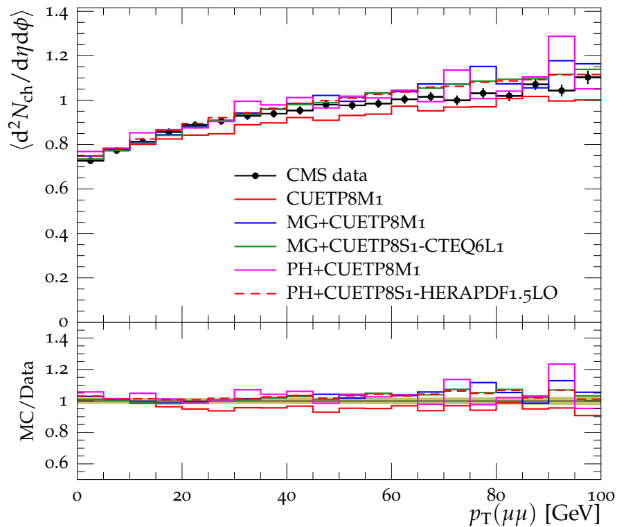
Transverse N_{\text{ch}} density vs p_{\text{T}}(\mu\mu)
