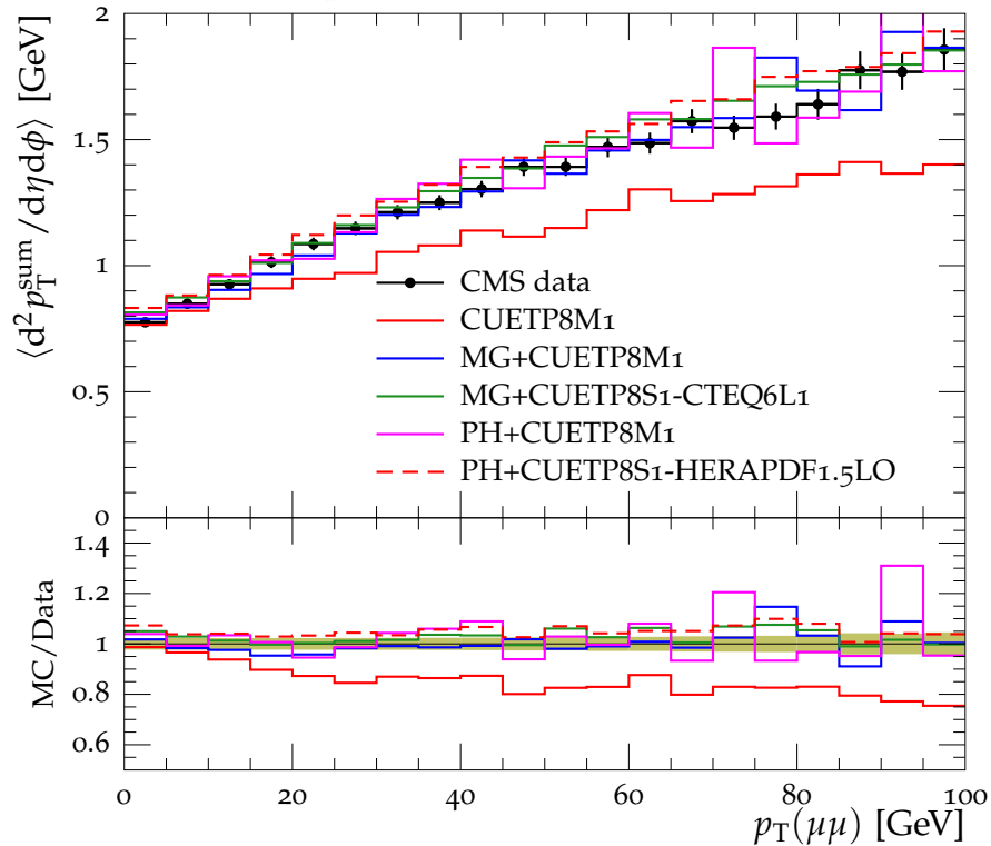
Transverse p_T^{\text{sum}} density vs p_T(\mu\mu)
