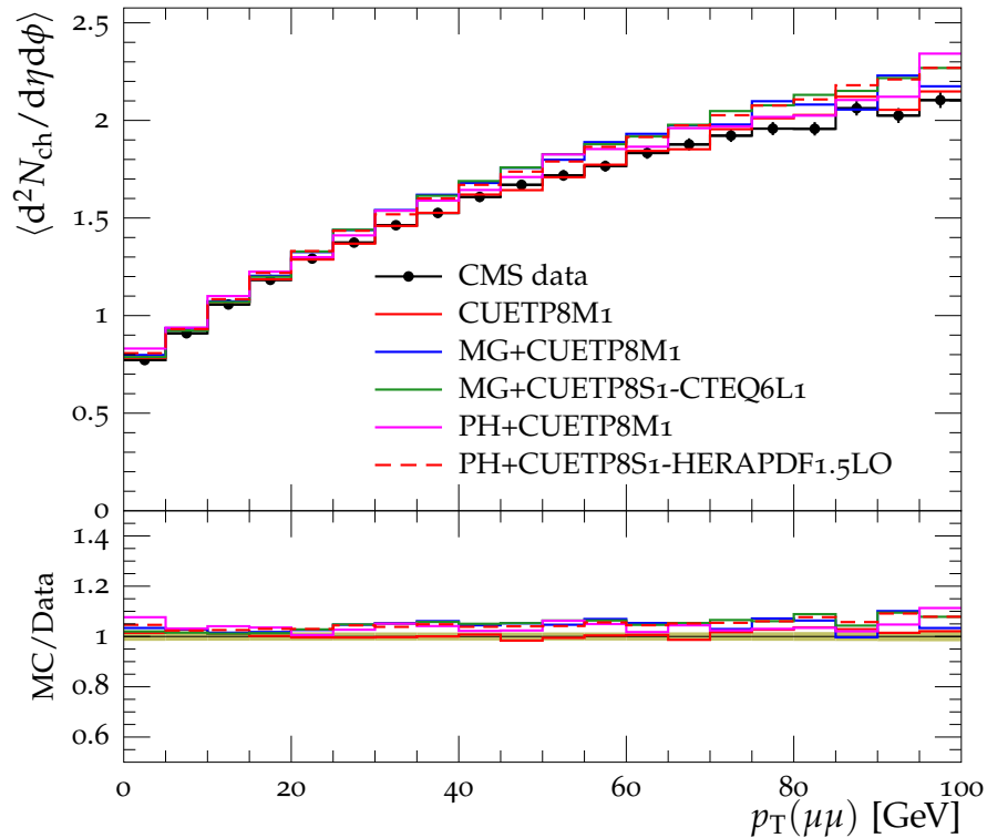
Away N_{\text{ch}} density vs p_{\text{T}}(\mu\mu)
