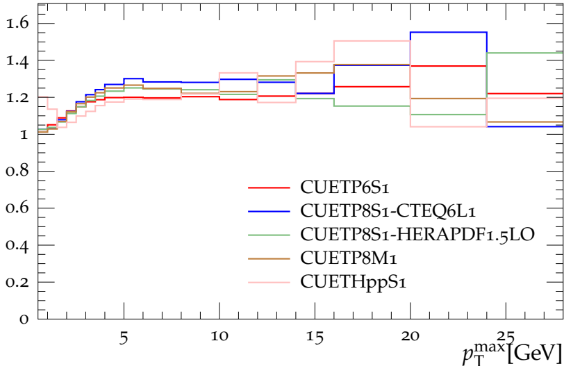
TransMAX charged p_T^{\text{sum}} density 13 TeV / 7 TeV
