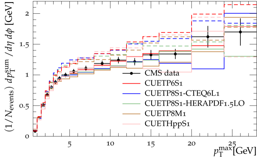
TransDIF charged p_T^{\text{sum}} density \sqrt{s} = 7 & 13 TeV
