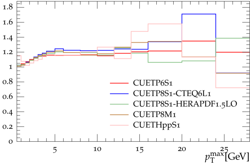
TransDIF charged p_T^{\text{sum}} density 13 TeV / 7 TeV
