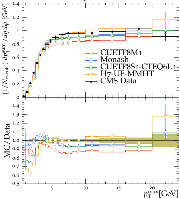
TransMIN charged-particle density, \sqrt{s} = 13 TeV
