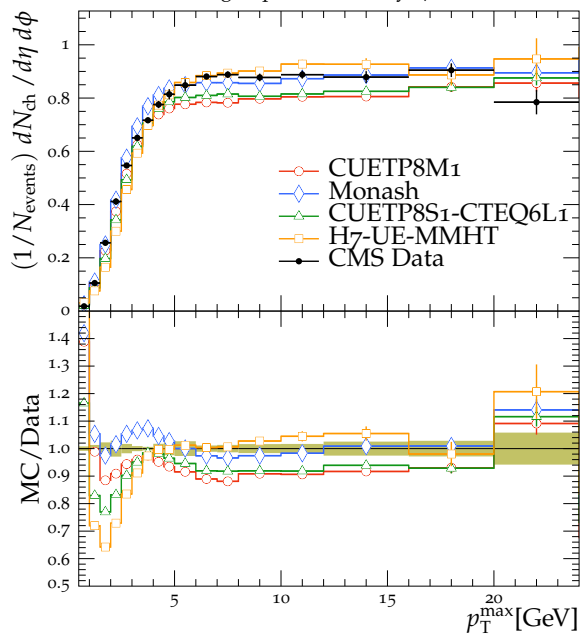
TransMIN charged-particle density, \sqrt{s} = 13 TeV
