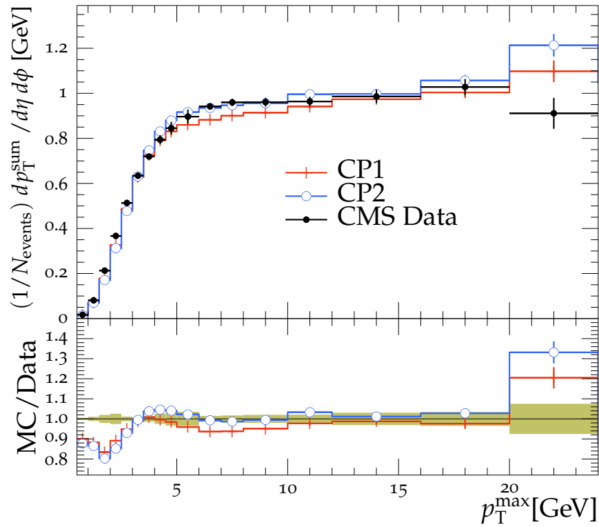
TransMIN charged p_T^{\text{sum}} density, \sqrt{s} = 13 TeV
