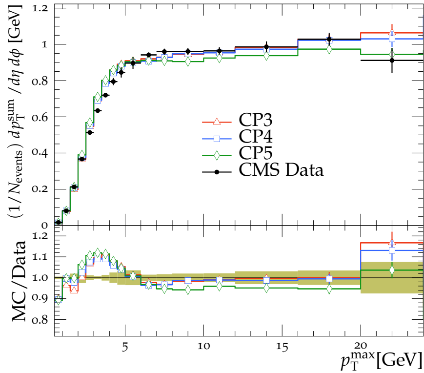
TransMIN charged p_T^{\text{sum}} density, \sqrt{s} = 13 \text{ TeV}
