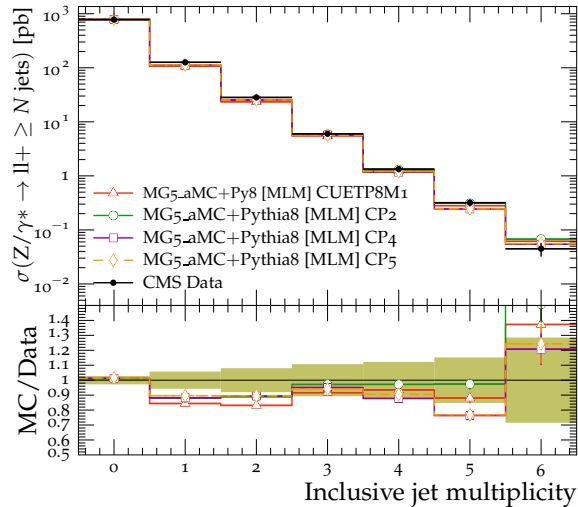
Z+jets, inclusive jet multiplicity, \sqrt{s} = 13 TeV
