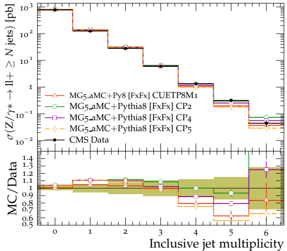
Z+jets, inclusive jet multiplicity, \sqrt{s} = 13 TeV
