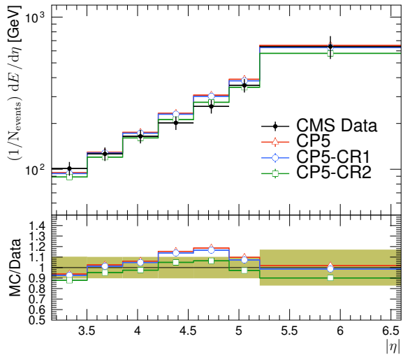
Energy density, NSD selection, \sqrt{s} = 13 TeV
