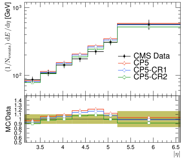
Energy density, inclusive selection, \sqrt{s} = 13 TeV
