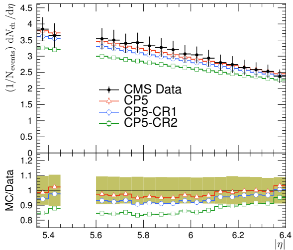
N_{\text{ch}} \geq 1 , p_{\text{T}} > 40 MeV, \sqrt{s} = 7 TeV
