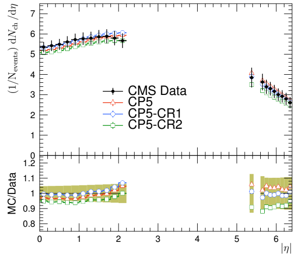
N_{\text{ch}} pseudorapidity distribution, \sqrt{s} = 8 TeV
