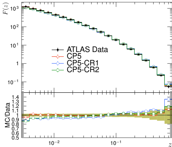
F(z) for 400 < p_T^{\text{jet}} < 500 GeV, \sqrt{s} = 7 TeV
