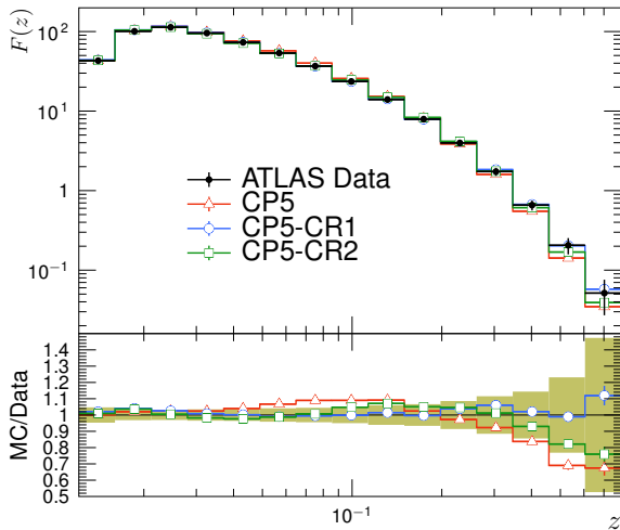
F(z) for 25 < p_T^{\text{jet}} < 40 GeV, \sqrt{s} = 7 TeV
