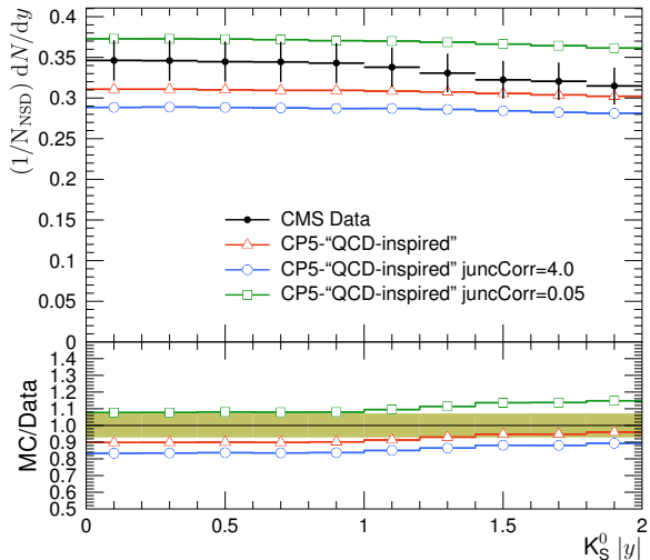
K_S^0 rapidity distribution, \sqrt{s} = 7 TeV
