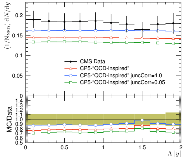
\Lambda rapidity distribution, \sqrt{s} = 7 TeV
