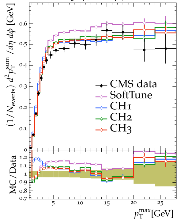
TransMin charged-particle density \sqrt{s} = 7 TeV
