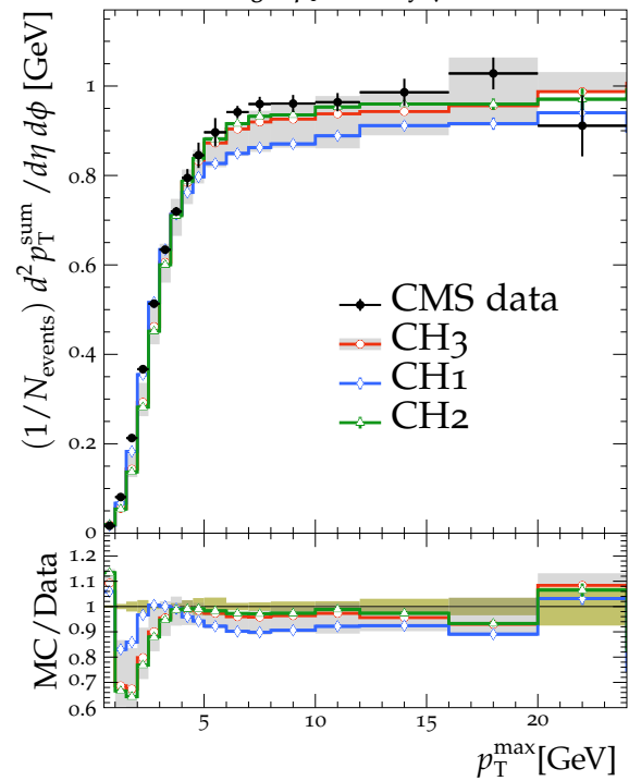
TransMin charged-particle density \sqrt{s} = 13 TeV
