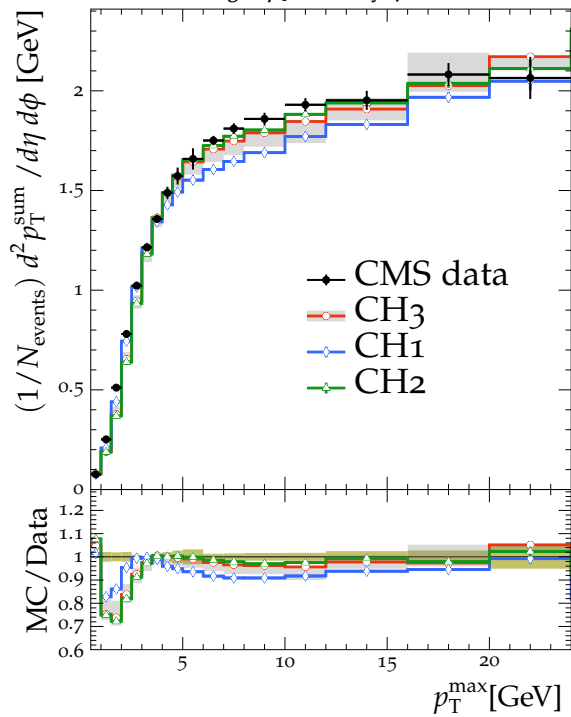
TransMax charged-particle density \sqrt{s} = 13 TeV
