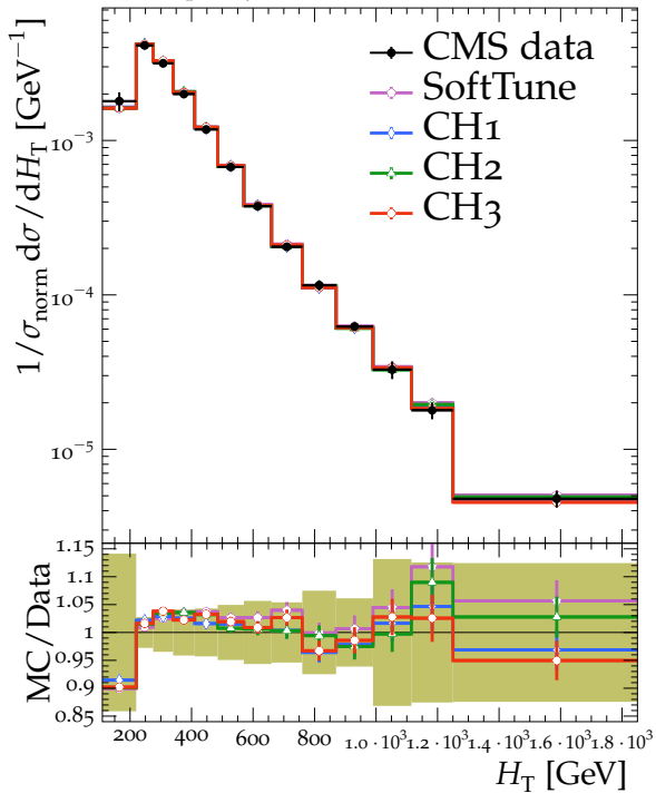
H_T in lepton+jets t\bar{t} events, \sqrt{s} = 13 TeV
