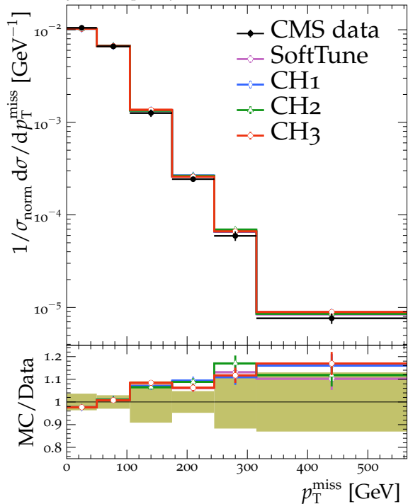
p_T^{\text{miss}} in lepton+jets t\bar{t} events, \sqrt{s} = 13 TeV
