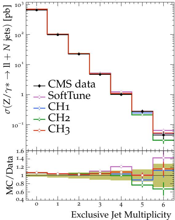
Z+jets, exclusive jet multiplicity, \sqrt{s} = 13 TeV
