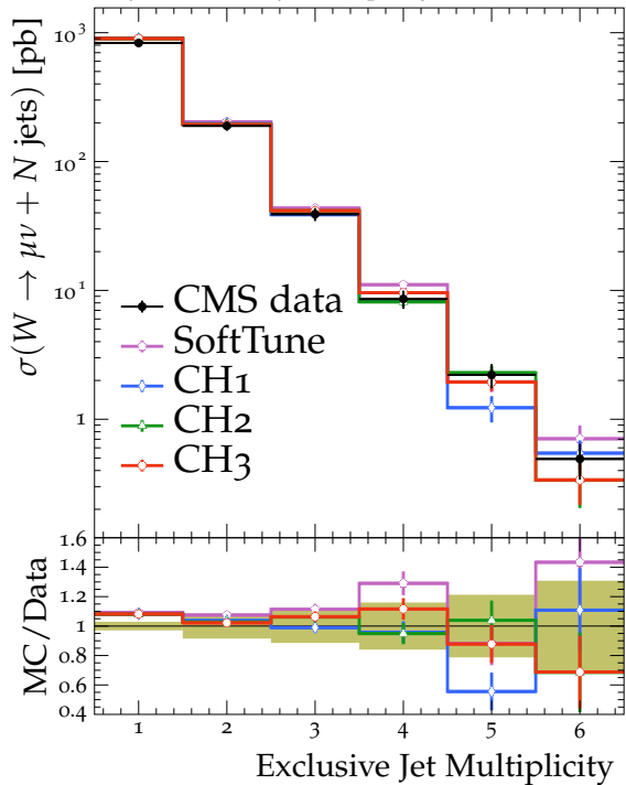
W+jets, exclusive jet multiplicity, \sqrt{s} = 13 TeV
