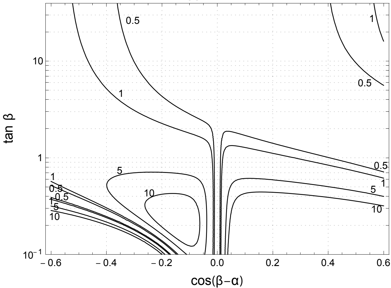
TYPE I 2HDM \sigma\mathcal{B}(gg\rightarrow H\rightarrow hh) (pb), m_H=300 GeV
