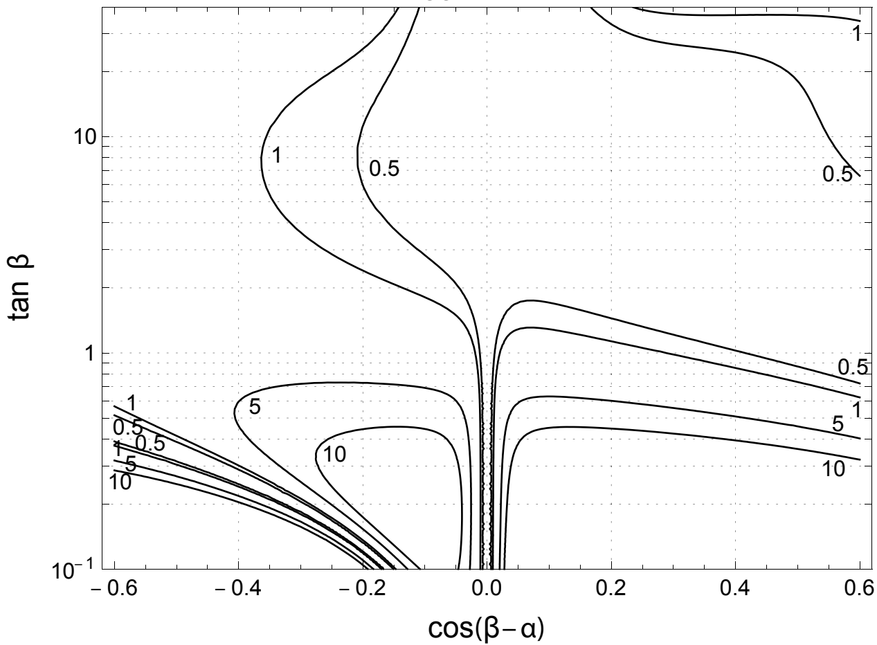
TYPE II 2HDM \sigma\mathcal{B}(gg\rightarrow H\rightarrow hh) (pb), m_H=300 GeV
