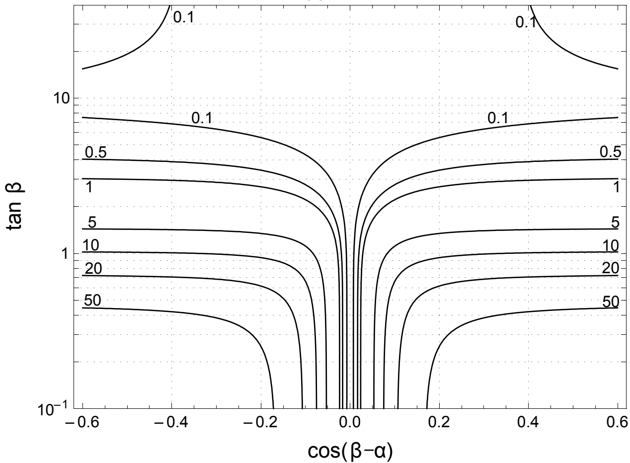
TYPE II 2HDM \sigma \mathcal{B}(gg \rightarrow A \rightarrow Zh) (pb), m_A = 300 GeV
