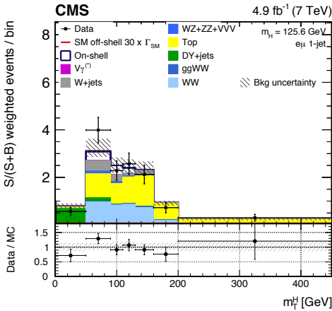
(c) GF 1-jet on-shell
