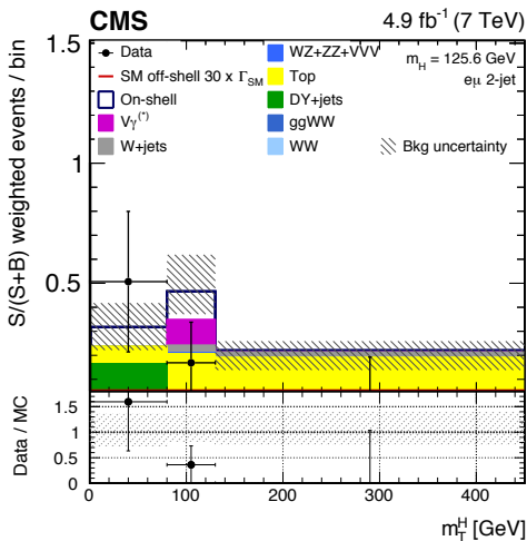
(e) VBF 2-jet on-shell
