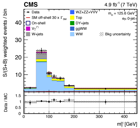
(b) GF 0-jet off-shell
