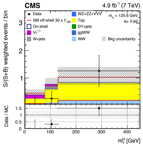
(f) VBF 2-jet off-shell
