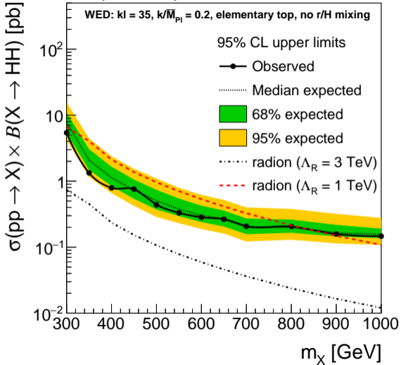
CMS, HH \rightarrow bb\tau\tau , 18.3 \text{ fb}^{-1} at \sqrt{s} = 8 \text{ TeV}
