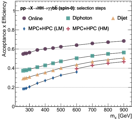
CMS Simulation (13 TeV)
