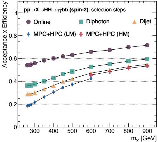
CMS Simulation (13 TeV)
