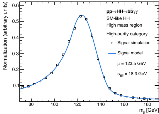
CMS Simulation (13 TeV)
