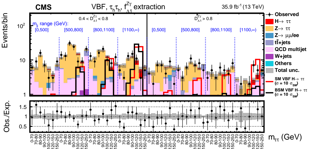
Observed and expected distributions in the VBF category in bins of m_{\tau\tau} , m_{JJ} , and D_{\Delta 1}^{Z\gamma} in the f_{\Delta 1}^{Z\gamma} analysis for the e\mu + e\tau_h + \tau_h\tau_h (upper) and \tau_h\tau_h (middle and lower) decay channels.
