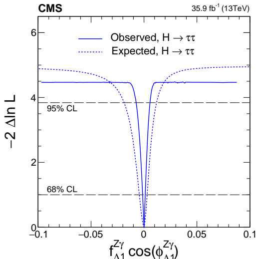
Observed (solid) and expected (dashed) likelihood scans of f_{a3} \cos(\phi_{a3}) (top left), f_{a2} \cos(\phi_{a2}) (top right), f_{\Lambda 1} \cos(\phi_{\Lambda 1}) (bottom left), and f_{\Lambda 1}^{Z\gamma} \cos(\phi_{\Lambda 1}^{Z\gamma}) (bottom right).
