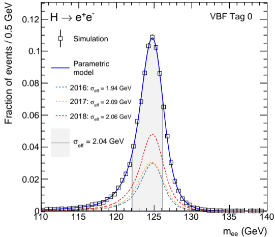
CMS Simulation (13 TeV)
