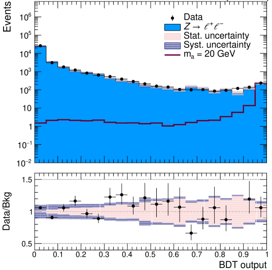
CMS 138 fb -1 (13 TeV)
