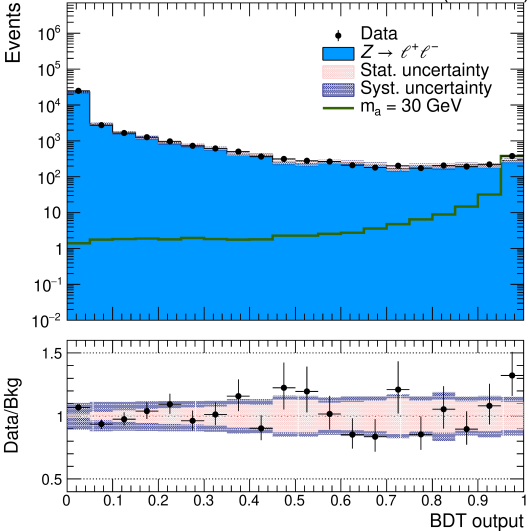
CMS 138 fb -1 (13 TeV)
