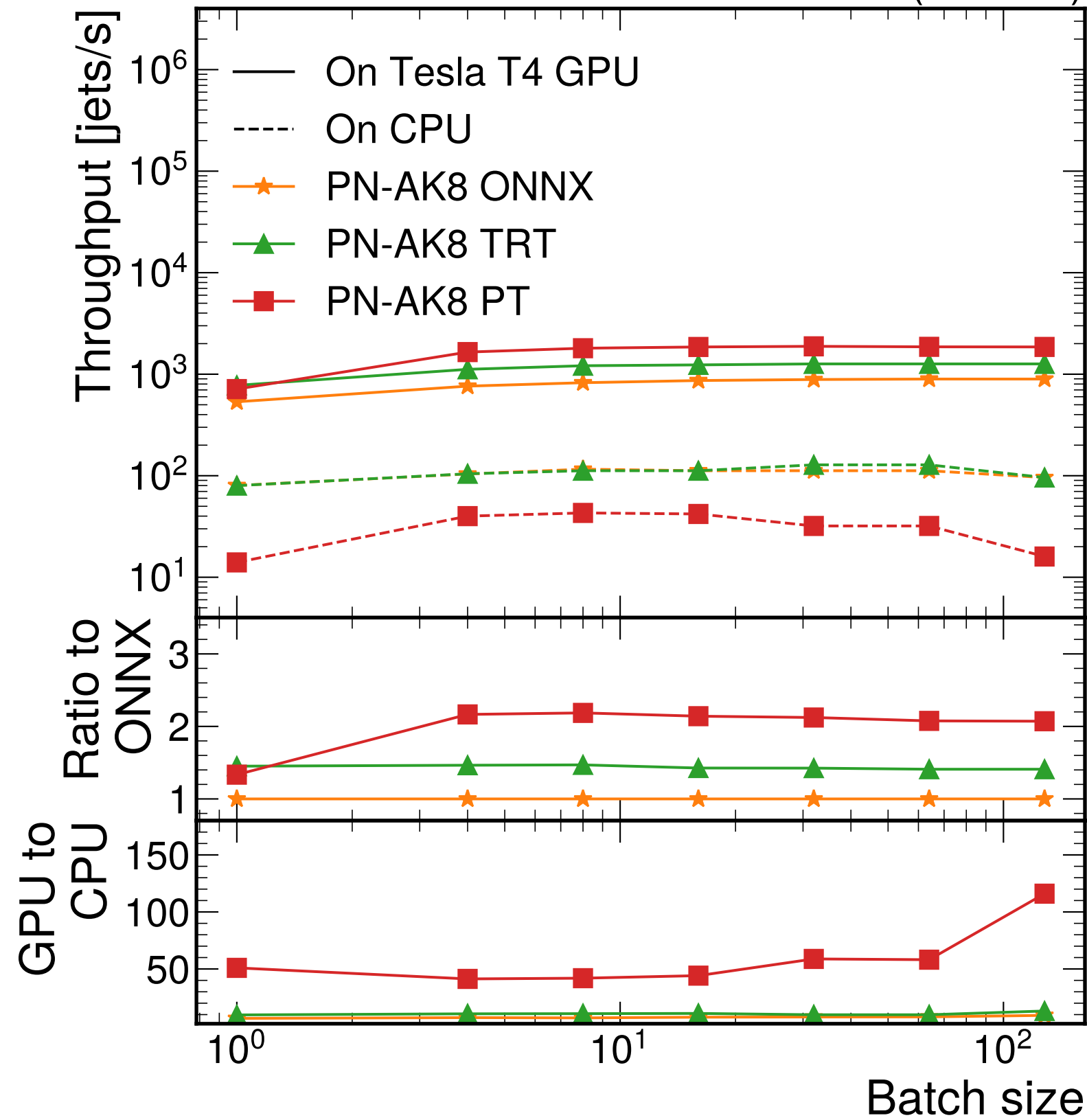
CMS Simulation (13 TeV)
