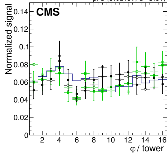
(a) Proton-lead collisions at \sqrt{s_{NN}} = 5.02 TeV recorded in 2013 and 2016 at B = 3.8 T.
