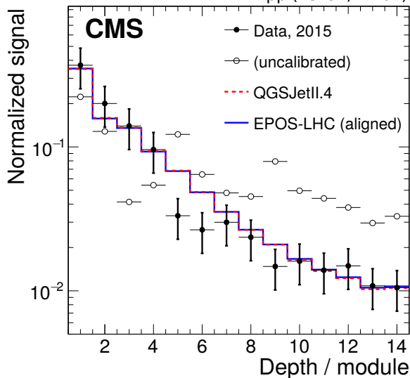
(b) Proton-proton collisions at \sqrt{s} = 13 TeV from 2015 at B = 0 T.
