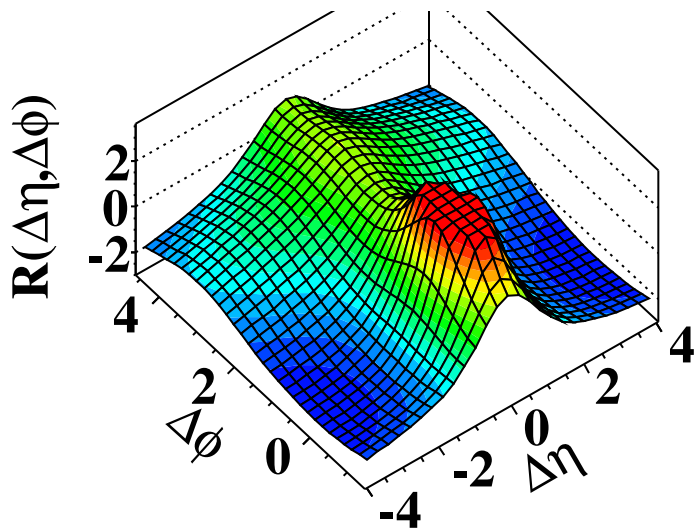
(a) CMS MinBias, p_T > 0.1 \text{ GeV}/c
