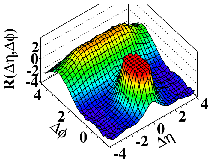
(c) CMS N \geq 110 , p_T > 0.1 \text{ GeV}/c
